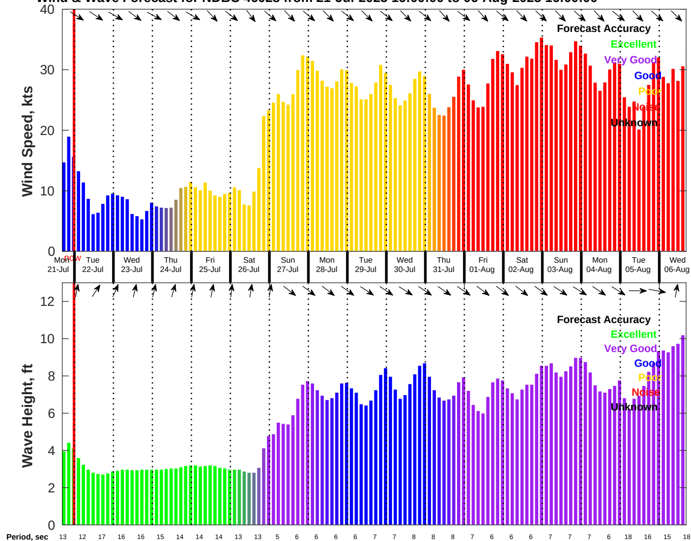
Wind & Wave Forecast for NDBC 46028 from 21-Jul-2025 16:00:00 to 06-Aug-2025 16:00:00
