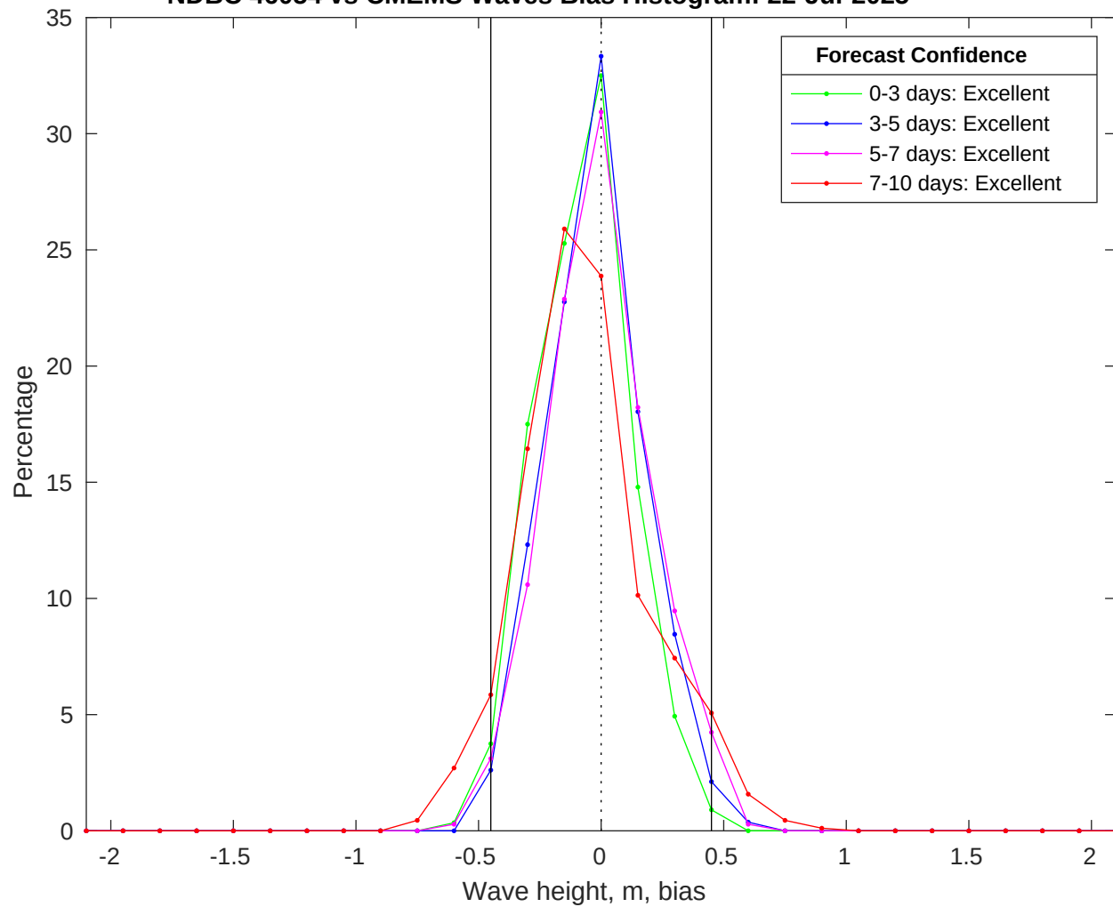
NDBC 46054 vs CMEMS Waves Bias Histogram: 22-Jul-2025
