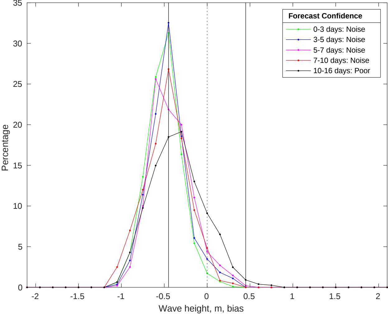
NDBC 46054 vs GFS Waves Bias Histogram: 22-Jul-2025
