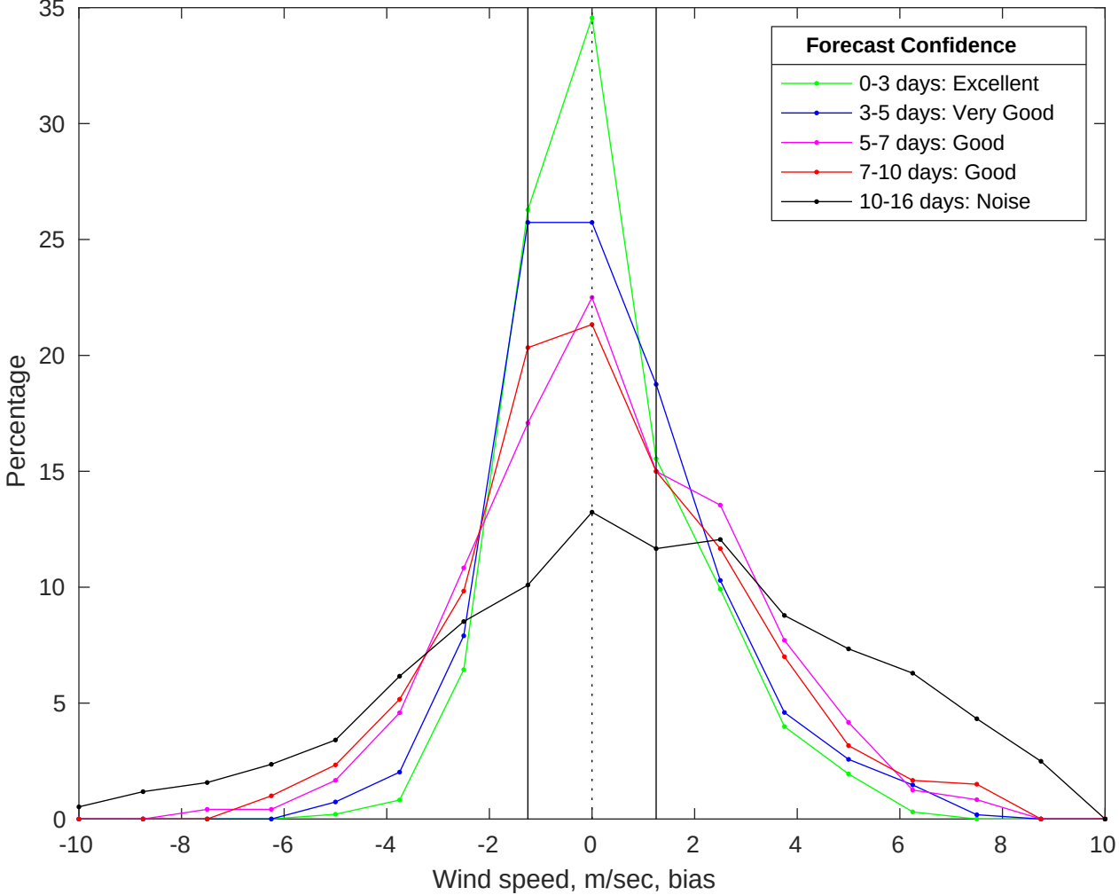
NDBC 46054 vs GFS Winds Bias Histogram: 22-Jul-2025
