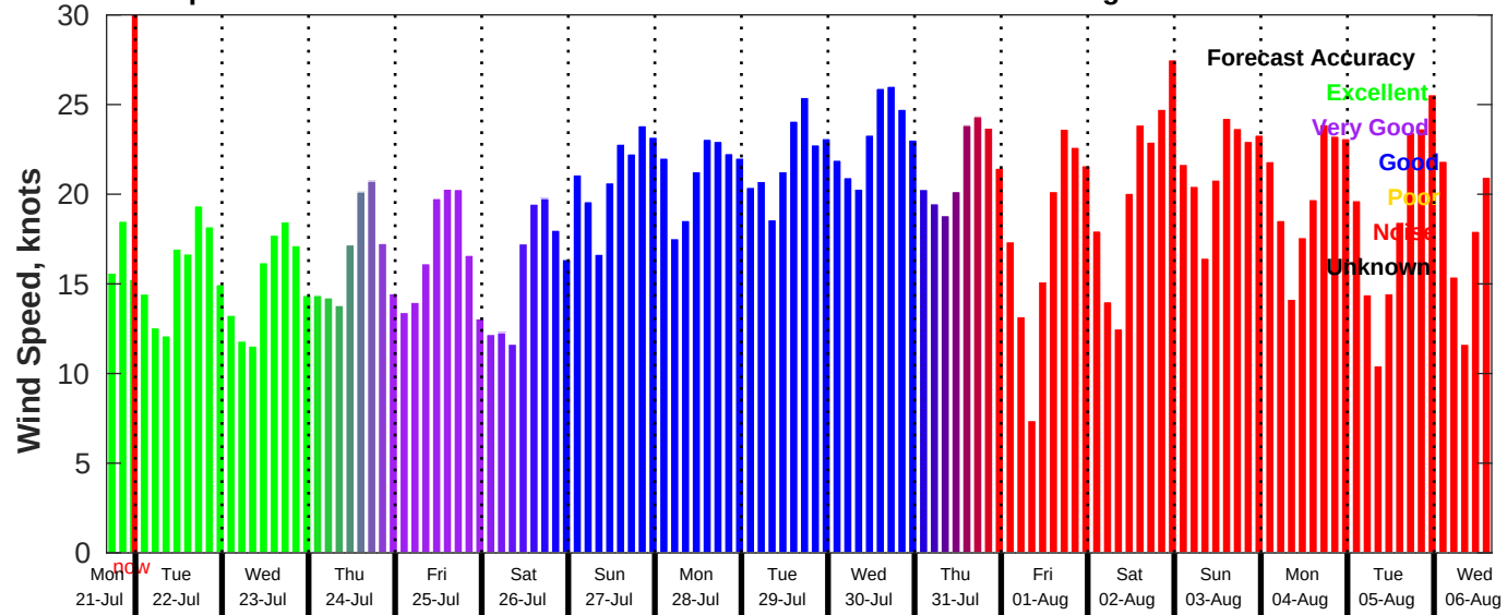
GFS Wind Speed Forecast for NDBC 46054 from 21-Jul-2025 16:00:00 to 06-Aug-2025 16:00:00
