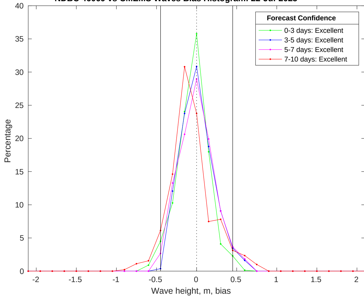
NDBC 46069 vs CMEMS Waves Bias Histogram: 22-Jul-2025
