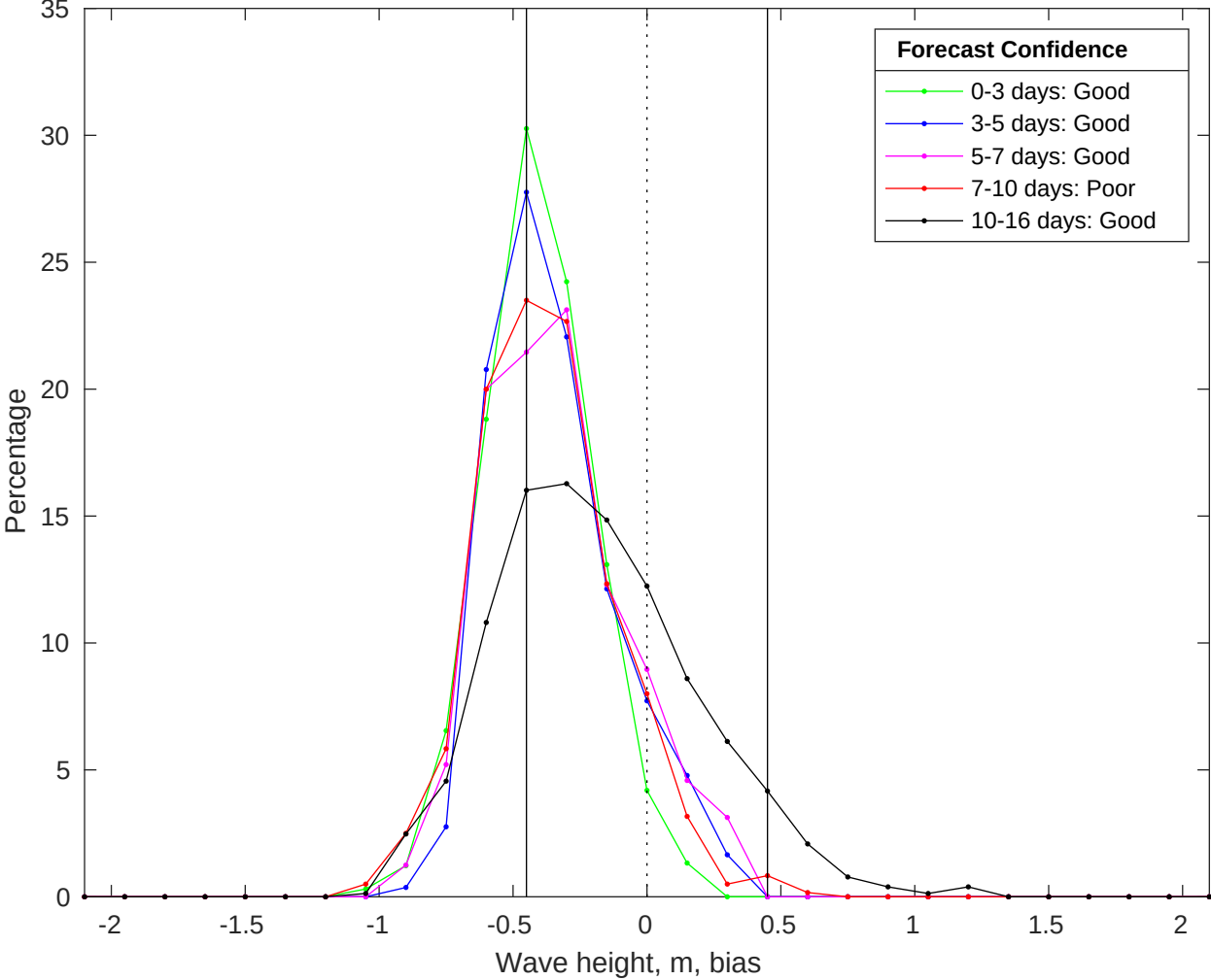
NDBC 46069 vs GFS Waves Bias Histogram: 22-Jul-2025
