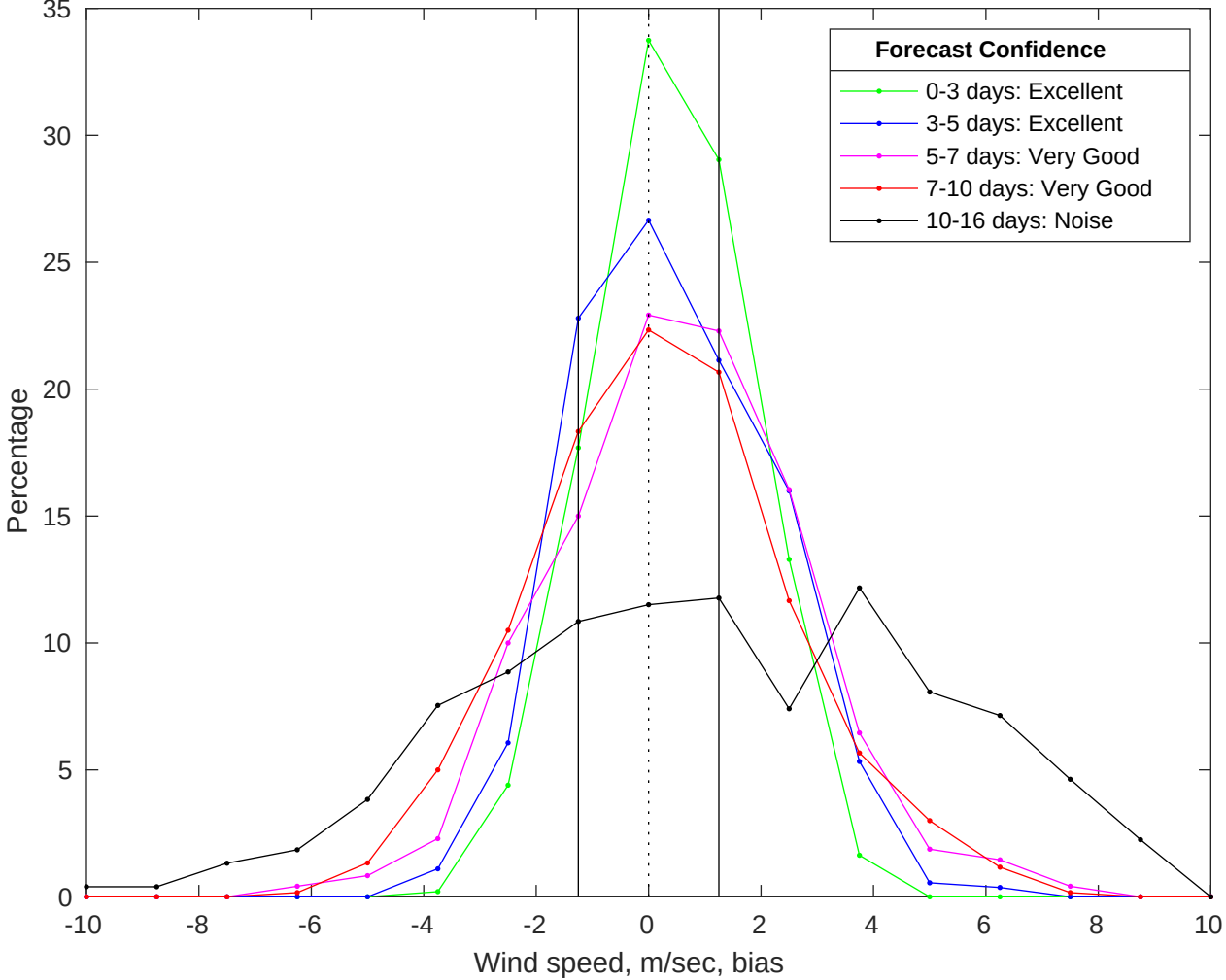
NDBC 46069 vs GFS Winds Bias Histogram: 22-Jul-2025
