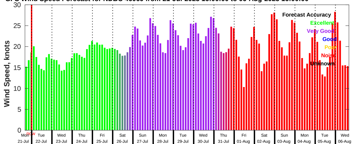
GFS Wind Speed Forecast for NDBC 46069 from 21-Jul-2025 16:00:00 to 06-Aug-2025 16:00:00
