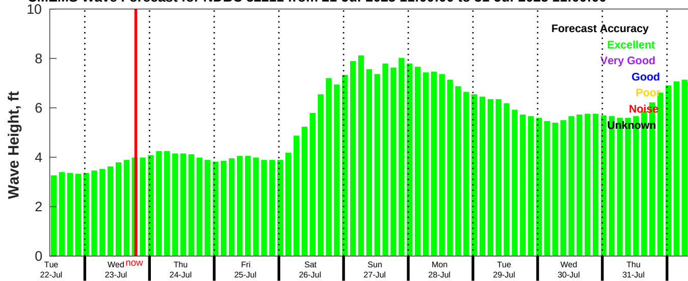
CMEMS Wave Forecast for NDBC 52211 from 21-Jul-2025 11:00:00 to 31-Jul-2025 11:00:00
