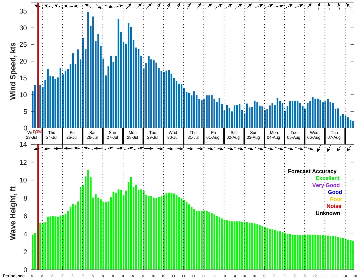
Wind & Wave Forecast for NDBC 52211 from 22-Jul-2025 11:00:00 to 07-Aug-2025 11:00:00
