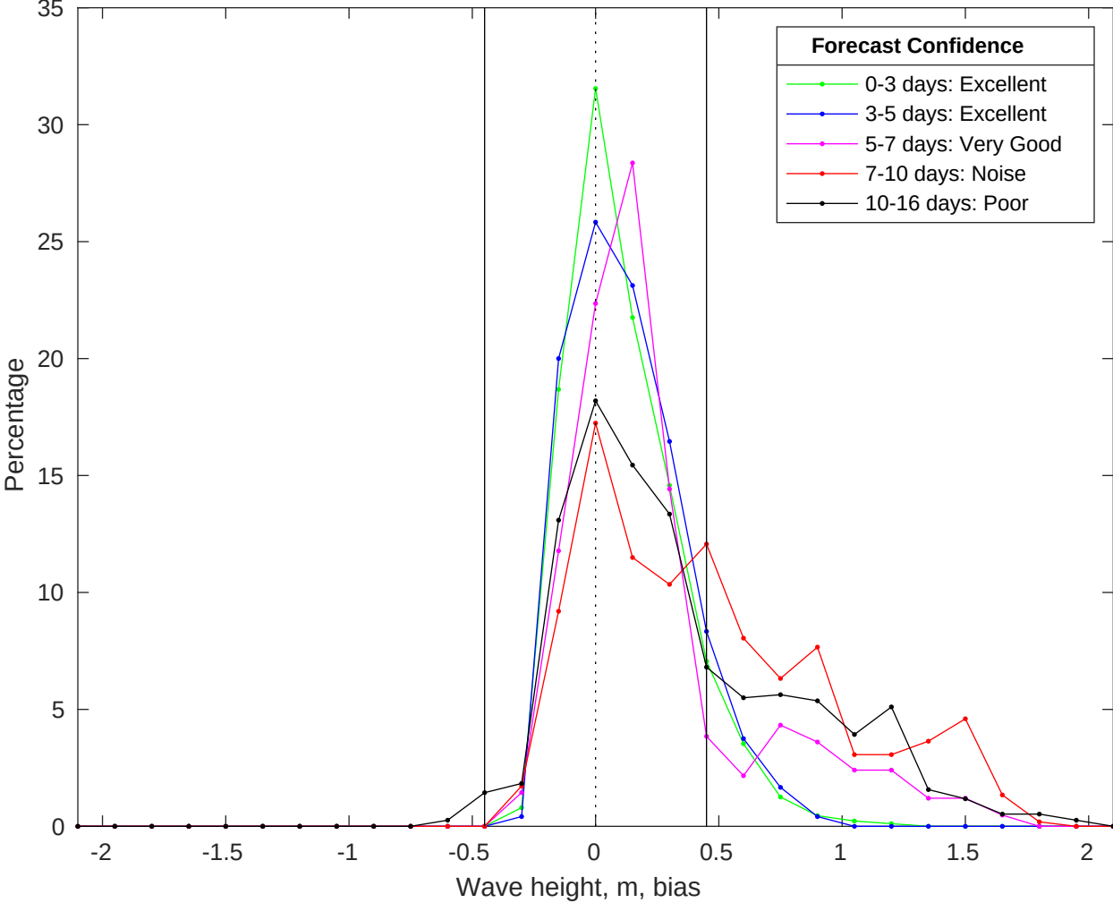
NDBC 52212 vs GFS Waves Bias Histogram: 22-Jul-2025
