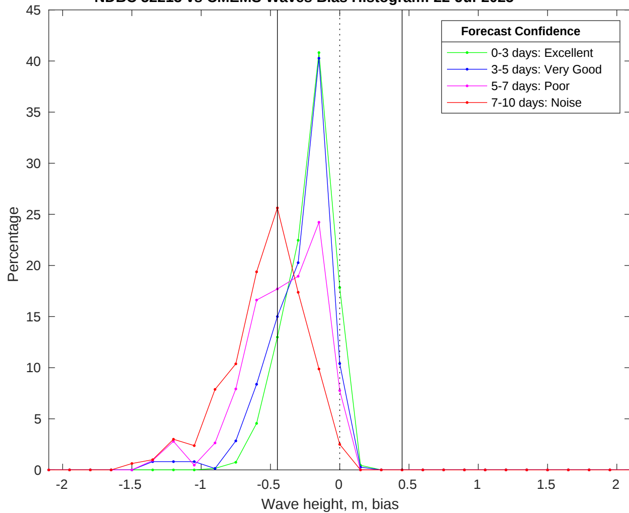
NDBC 52213 vs CMEMS Waves Bias Histogram: 22-Jul-2025
