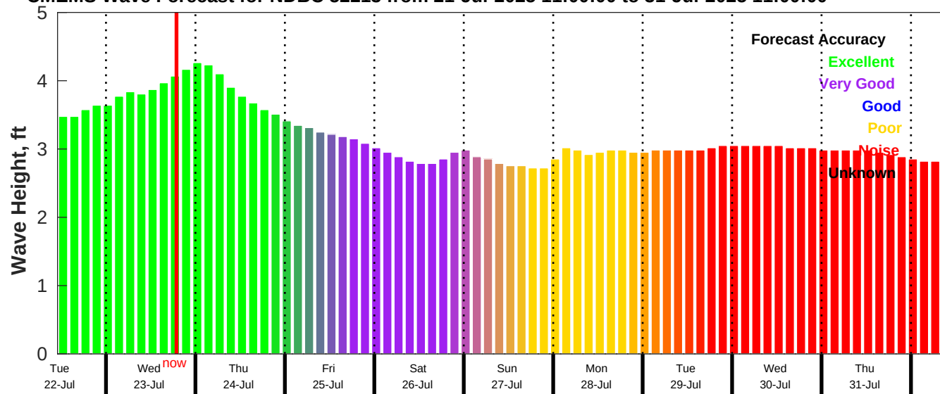
CMEMS Wave Forecast for NDBC 52213 from 21-Jul-2025 11:00:00 to 31-Jul-2025 11:00:00
