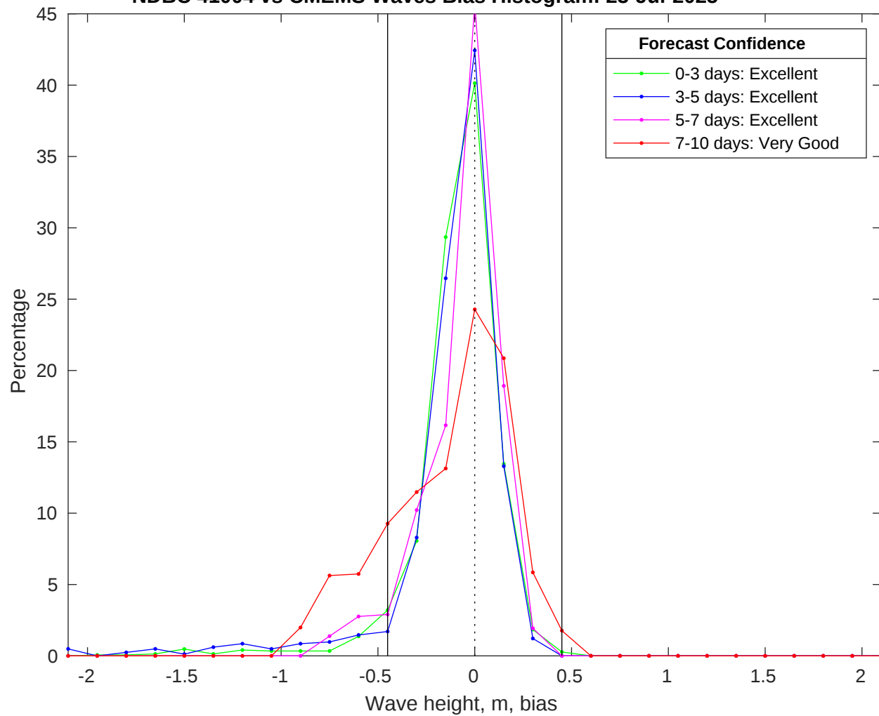
NDBC 41004 vs CMEMS Waves Bias Histogram: 23-Jul-2025
