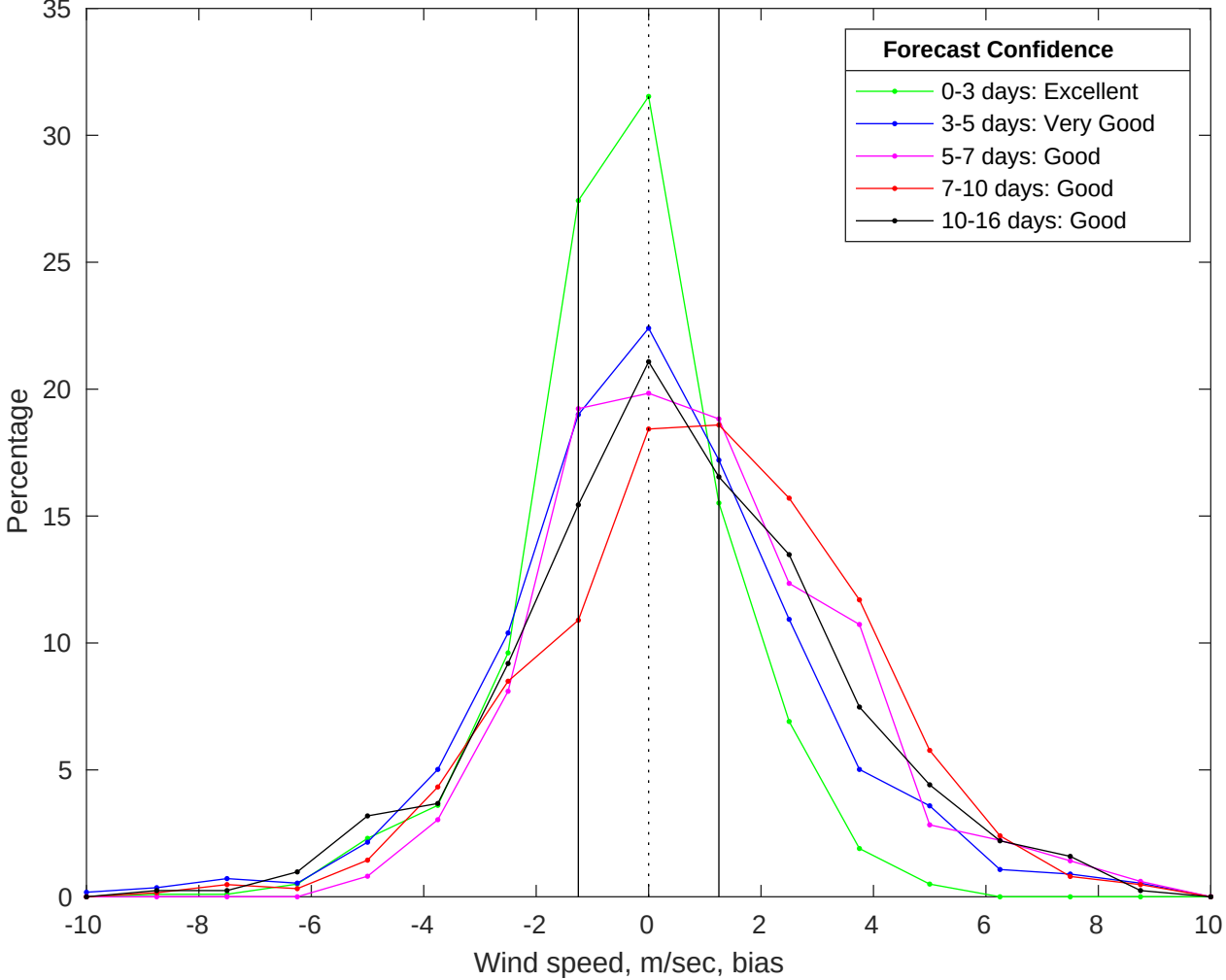
NDBC 41004 vs GFS Winds Bias Histogram: 23-Jul-2025
