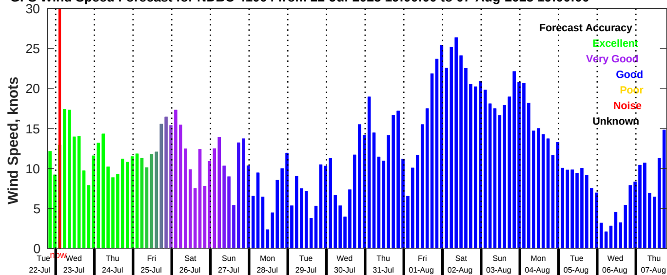
GFS Wind Speed Forecast for NDBC 41004 from 22-Jul-2025 19:00:00 to 07-Aug-2025 19:00:00
