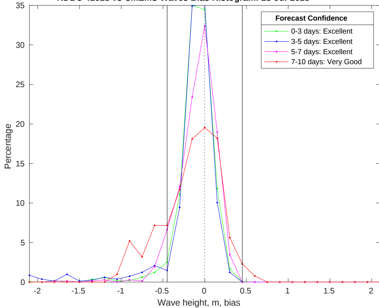
NDBC 41013 vs CMEMS Waves Bias Histogram: 23-Jul-2025
