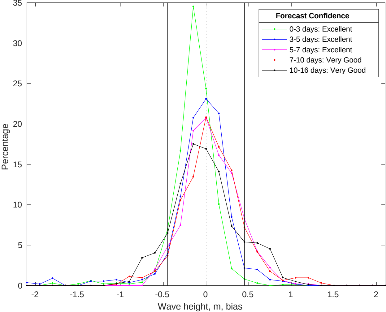
NDBC 41013 vs GFS Waves Bias Histogram: 23-Jul-2025
