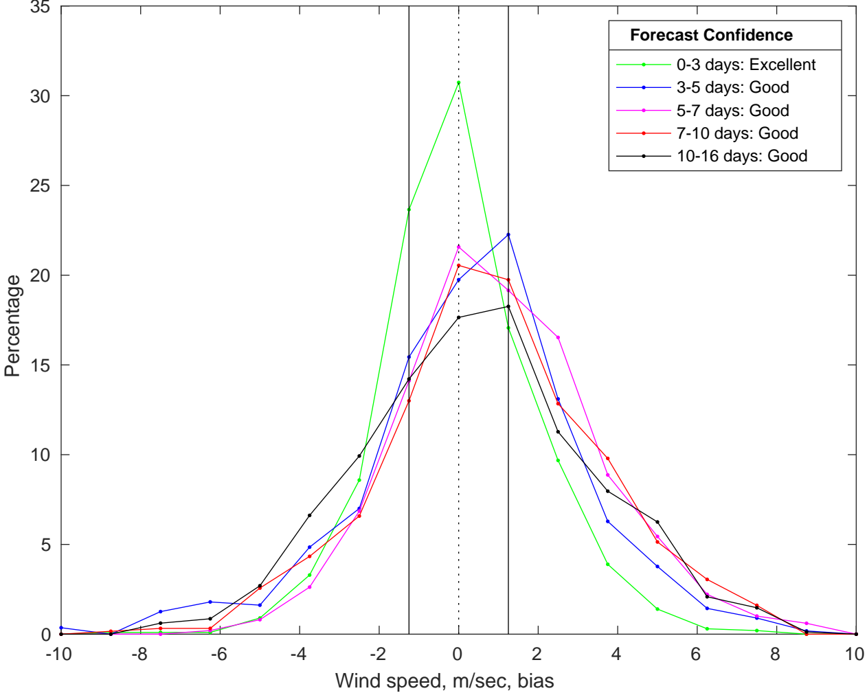
NDBC 41013 vs GFS Winds Bias Histogram: 23-Jul-2025
