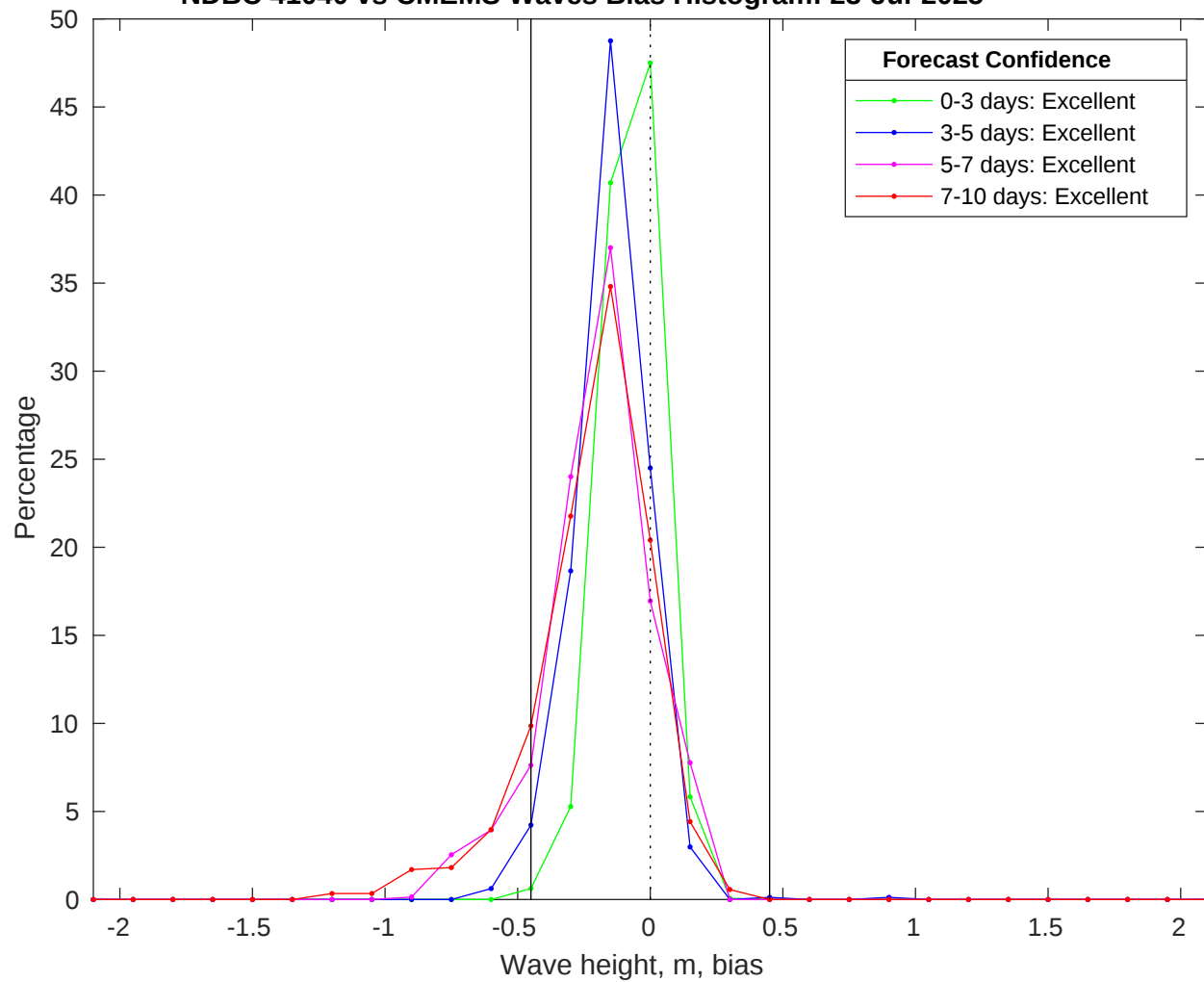
NDBC 41040 vs CMEMS Waves Bias Histogram: 23-Jul-2025
