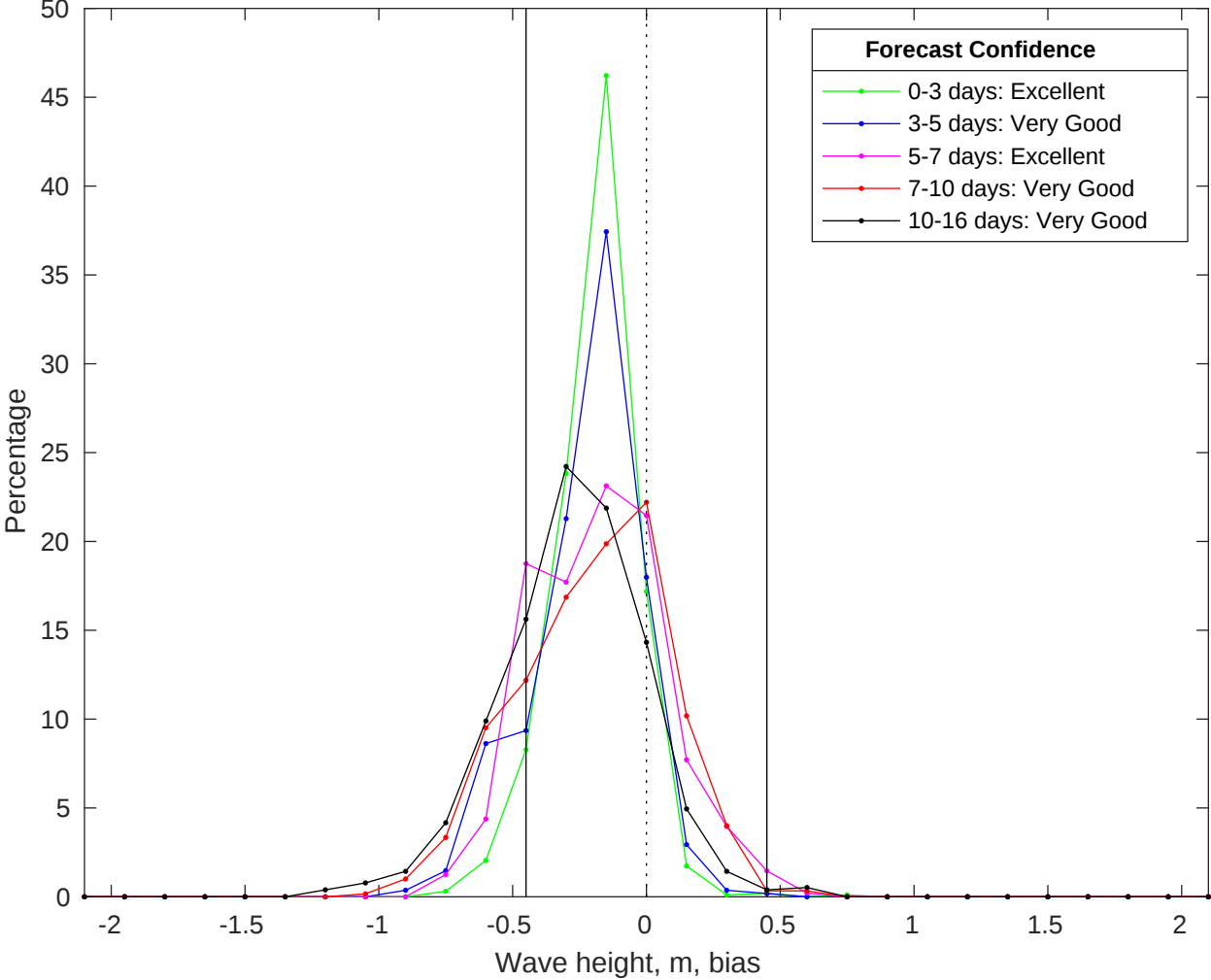
NDBC 41040 vs GFS Waves Bias Histogram: 23-Jul-2025
