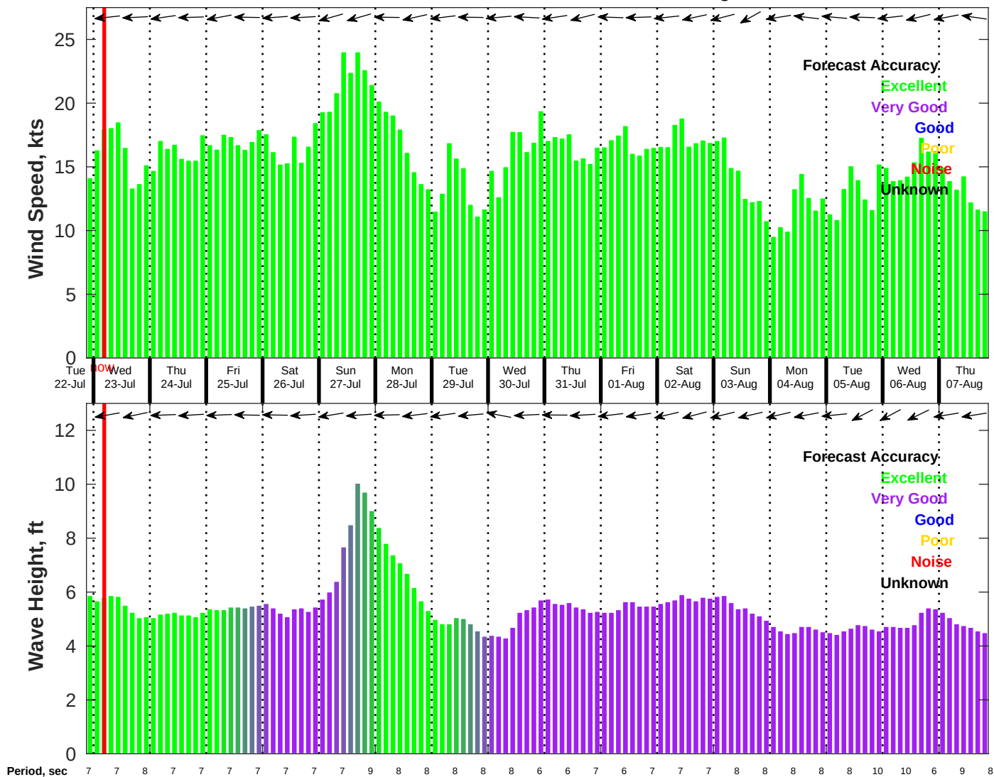
Wind & Wave Forecast for NDBC 41040 from 22-Jul-2025 21:00:00 to 07-Aug-2025 21:00:00
