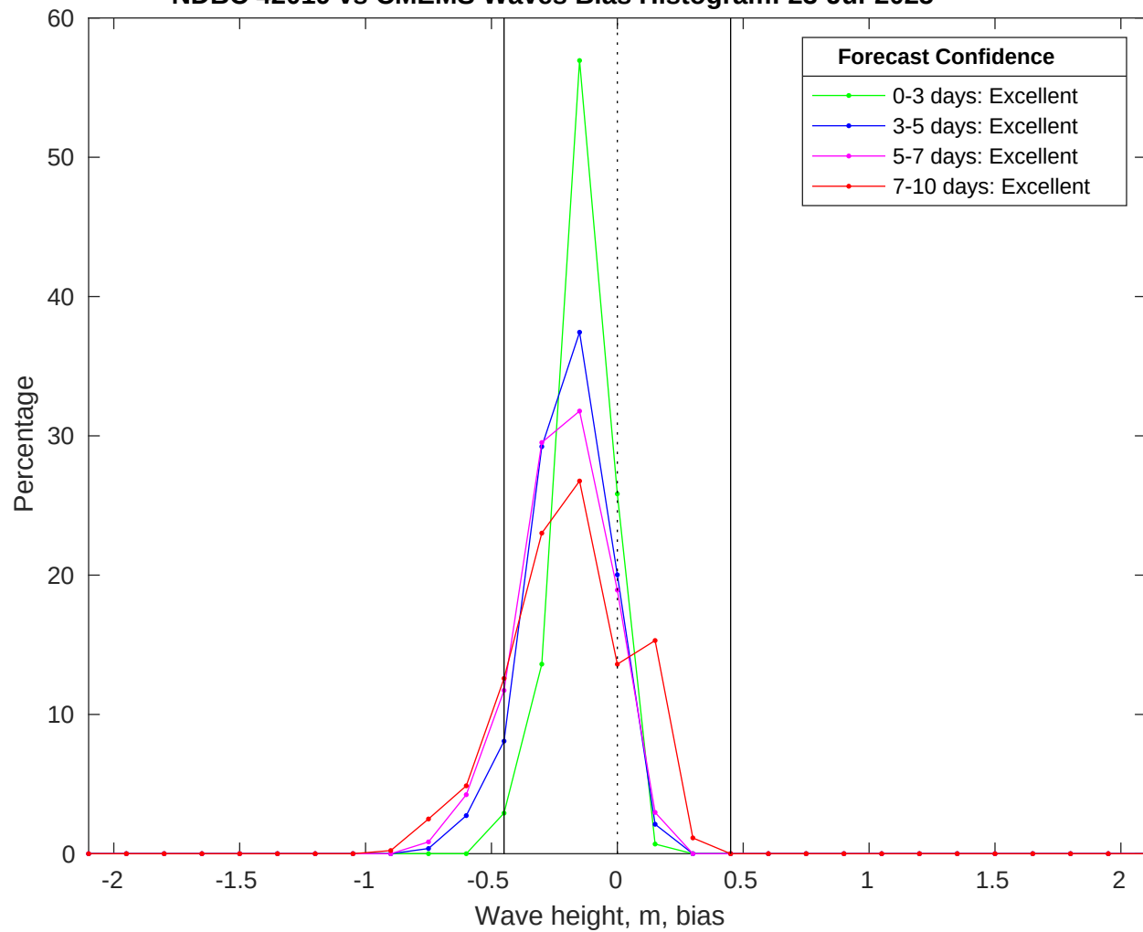
NDBC 42019 vs CMEMS Waves Bias Histogram: 23-Jul-2025
