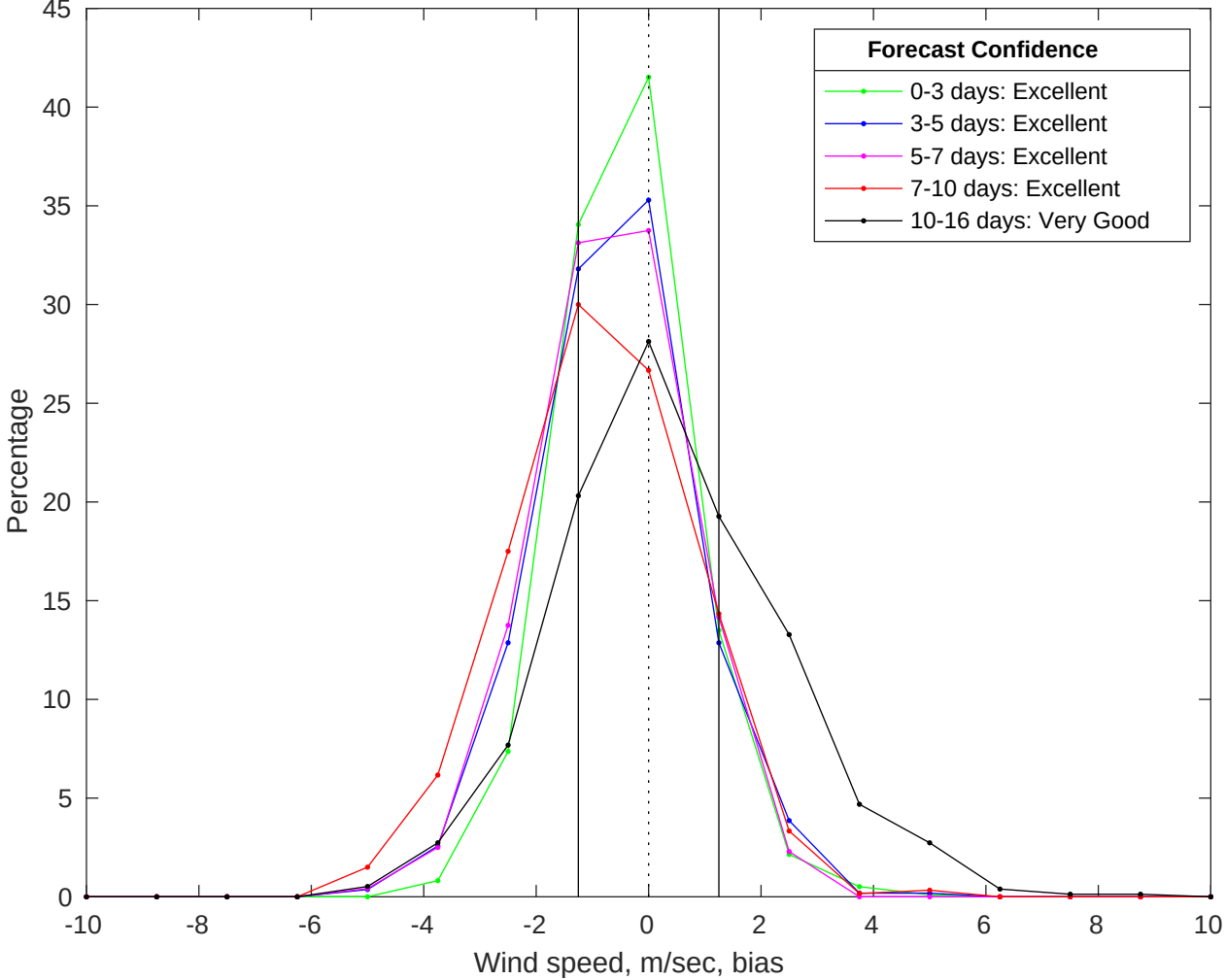
NDBC 42019 vs GFS Winds Bias Histogram: 23-Jul-2025
