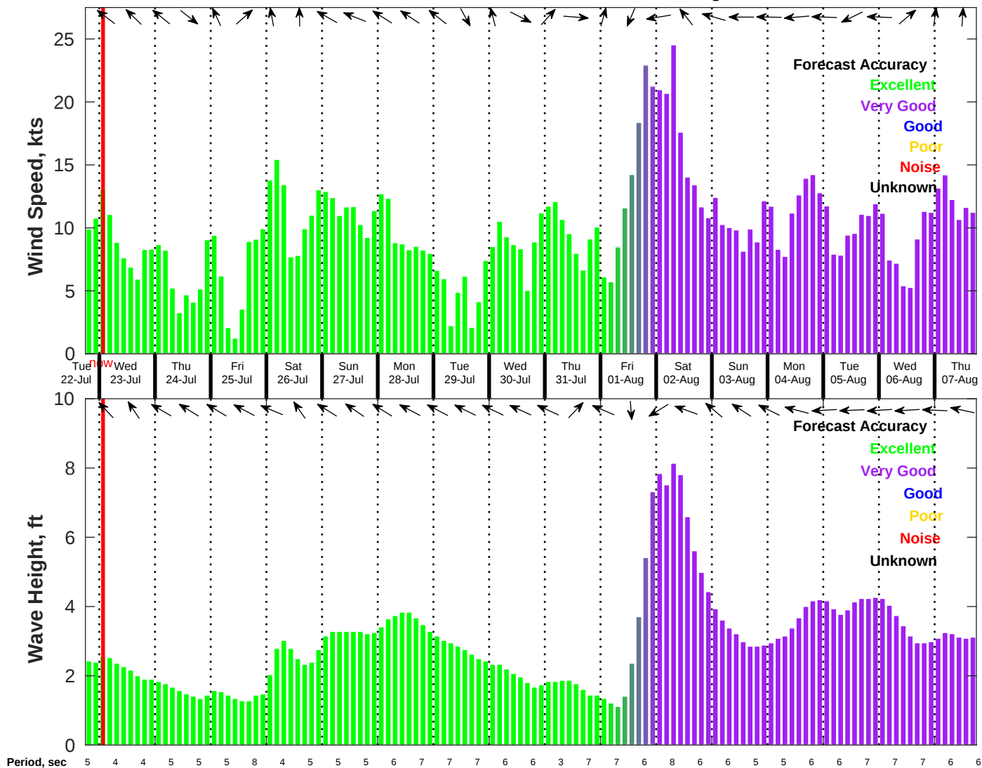
Wind & Wave Forecast for NDBC 42019 from 22-Jul-2025 18:00:00 to 07-Aug-2025 18:00:00
