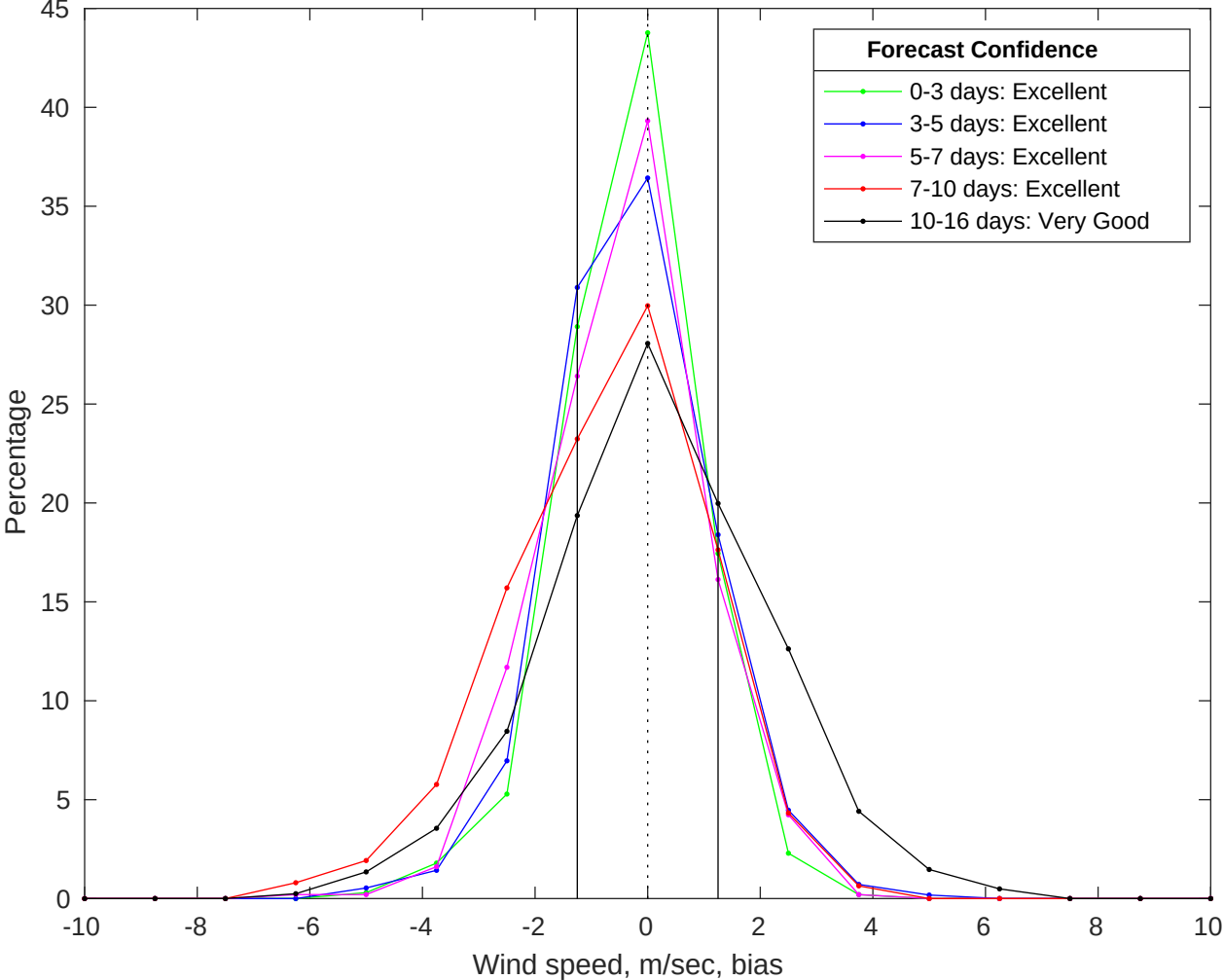
NDBC 42020 vs GFS Winds Bias Histogram: 23-Jul-2025
