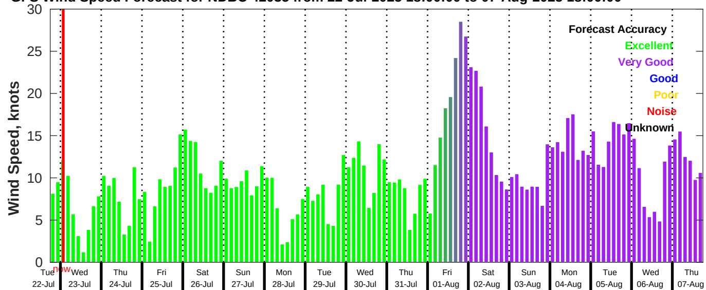
GFS Wind Speed Forecast for NDBC 42035 from 22-Jul-2025 18:00:00 to 07-Aug-2025 18:00:00
