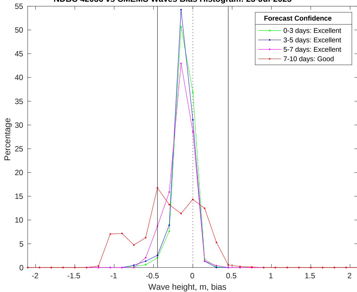
NDBC 42036 vs CMEMS Waves Bias Histogram: 23-Jul-2025
