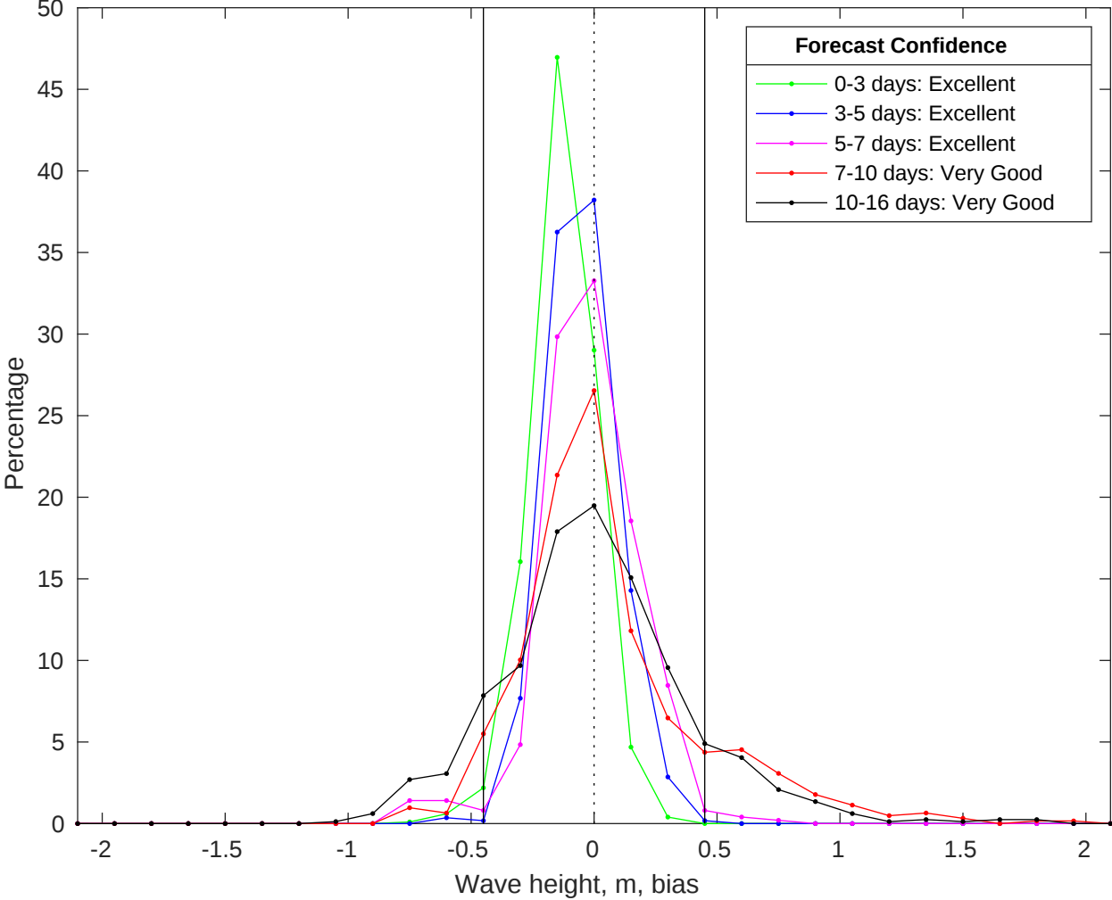
NDBC 42036 vs GFS Waves Bias Histogram: 23-Jul-2025
