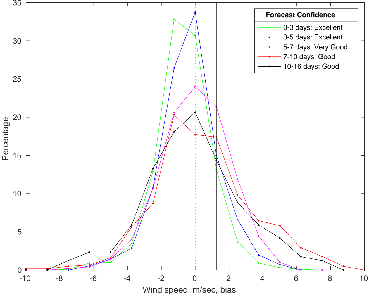
NDBC 42036 vs GFS Winds Bias Histogram: 23-Jul-2025
