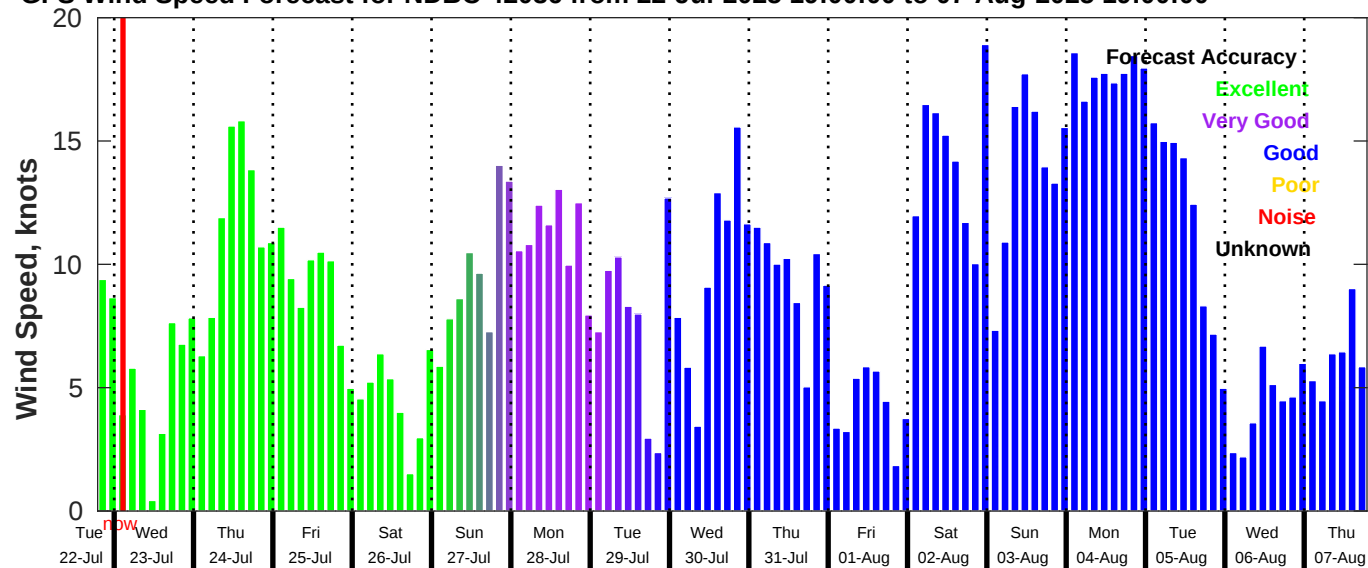
GFS Wind Speed Forecast for NDBC 42036 from 22-Jul-2025 19:00:00 to 07-Aug-2025 19:00:00
