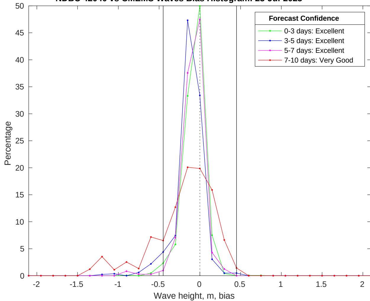
NDBC 42040 vs CMEMS Waves Bias Histogram: 23-Jul-2025
