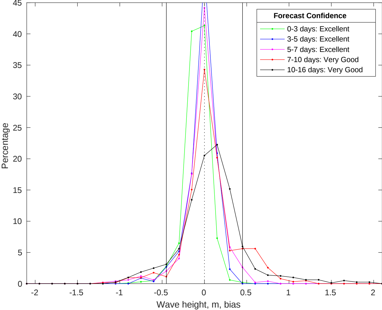
NDBC 42040 vs GFS Waves Bias Histogram: 23-Jul-2025
