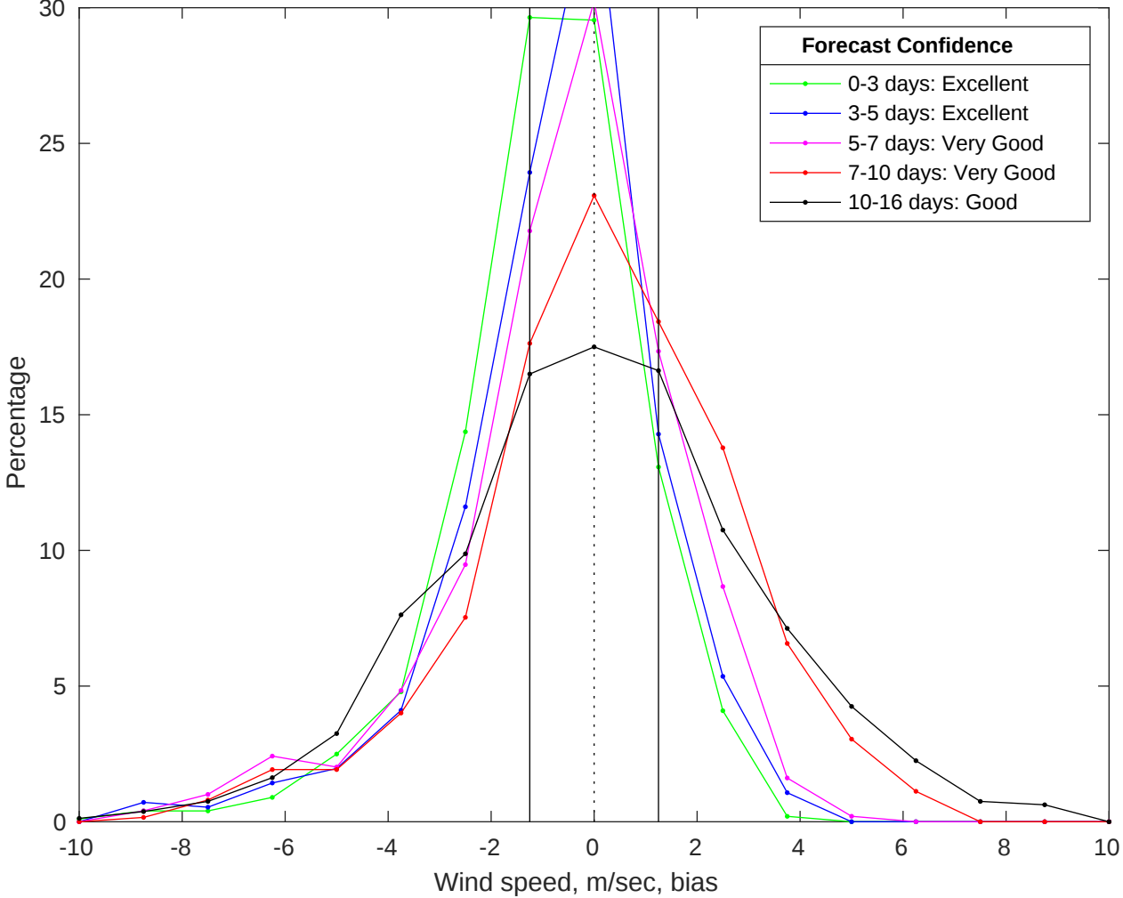
NDBC 42040 vs GFS Winds Bias Histogram: 23-Jul-2025
