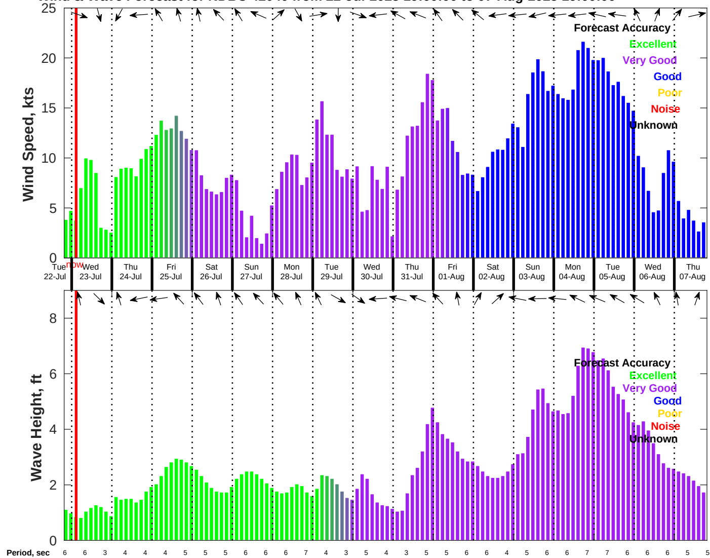
Wind & Wave Forecast for NDBC 42040 from 22-Jul-2025 19:00:00 to 07-Aug-2025 19:00:00
