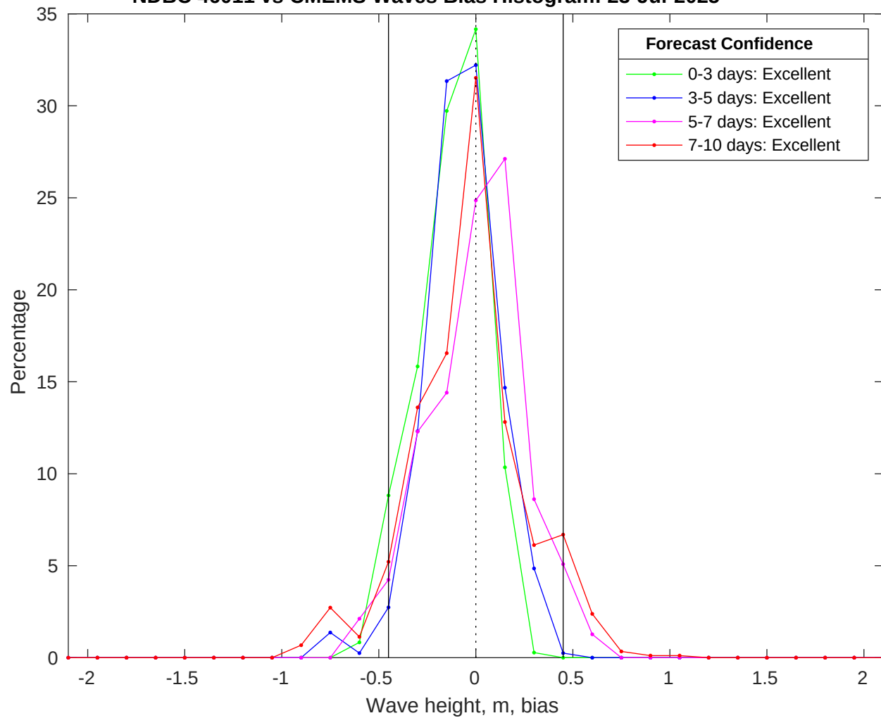
NDBC 46011 vs CMEMS Waves Bias Histogram: 23-Jul-2025
