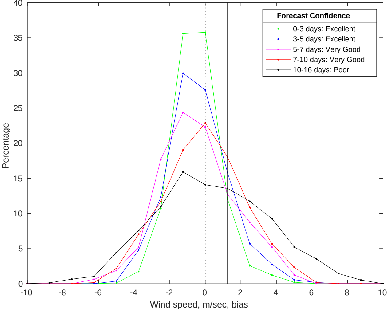
NDBC 46011 vs GFS Winds Bias Histogram: 23-Jul-2025
