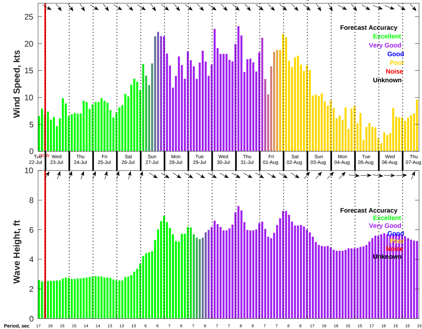
Wind & Wave Forecast for NDBC 46011 from 22-Jul-2025 16:00:00 to 07-Aug-2025 16:00:00
