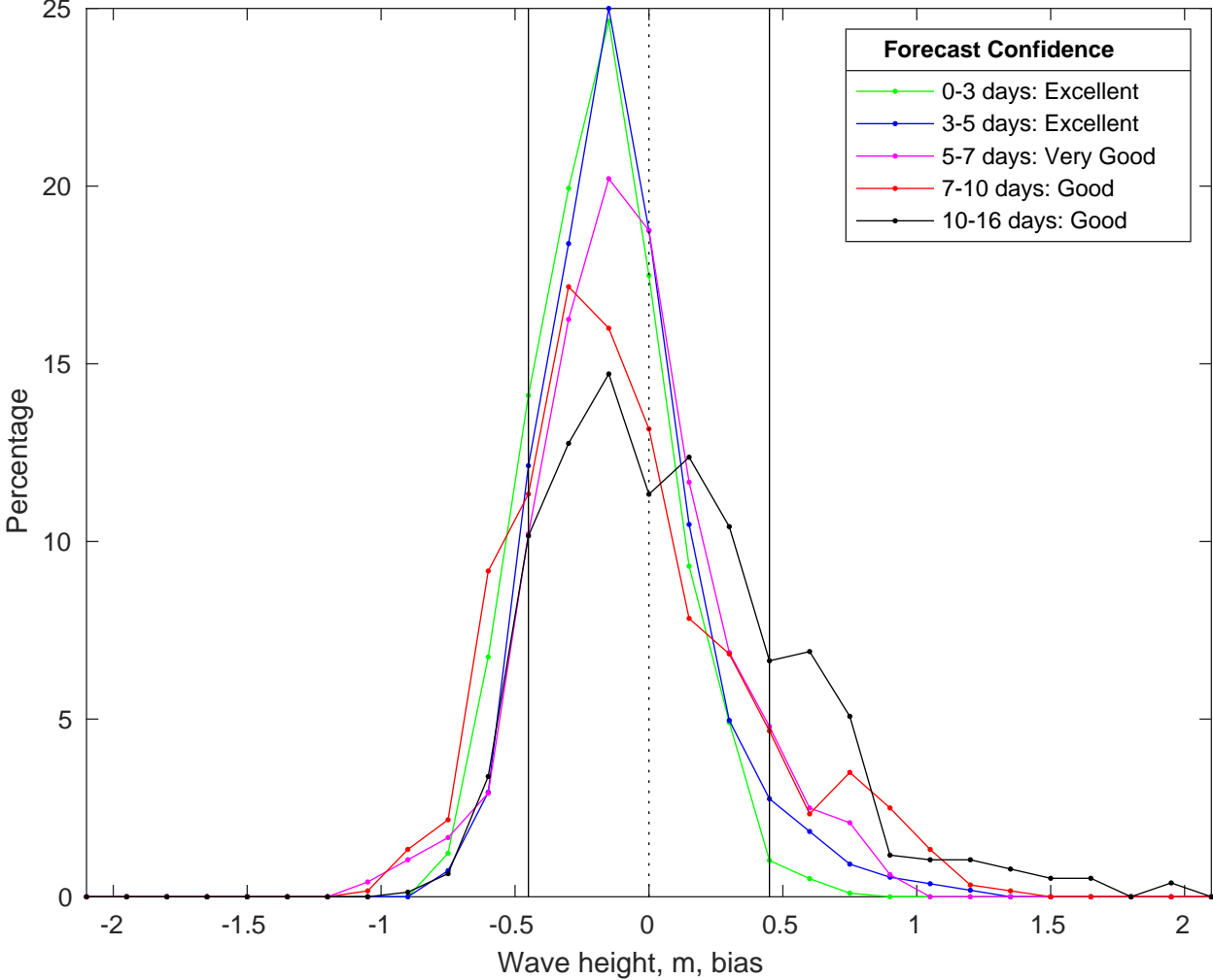
NDBC 46028 vs GFS Waves Bias Histogram: 23-Jul-2025
