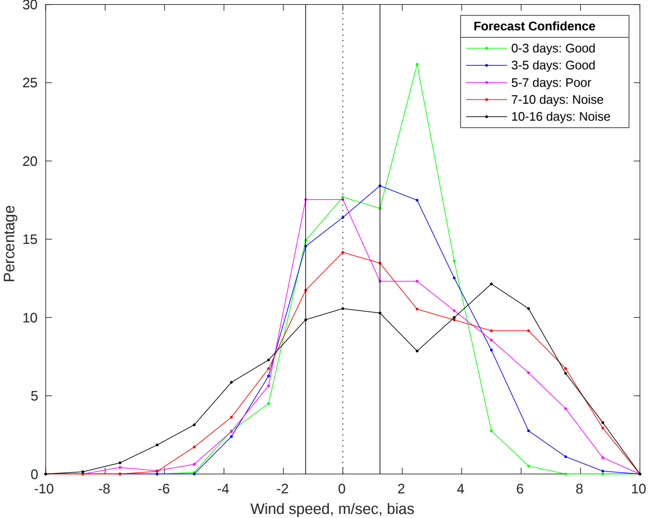
NDBC 46028 vs GFS Winds Bias Histogram: 23-Jul-2025
