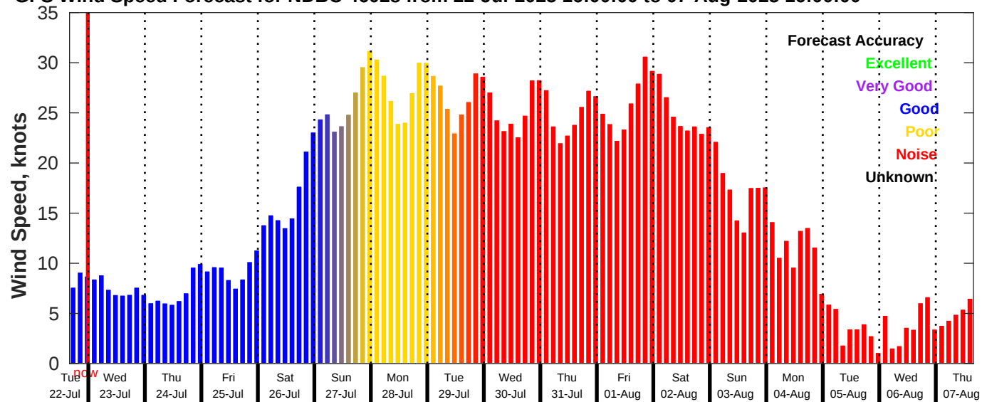
GFS Wind Speed Forecast for NDBC 46028 from 22-Jul-2025 16:00:00 to 07-Aug-2025 16:00:00
