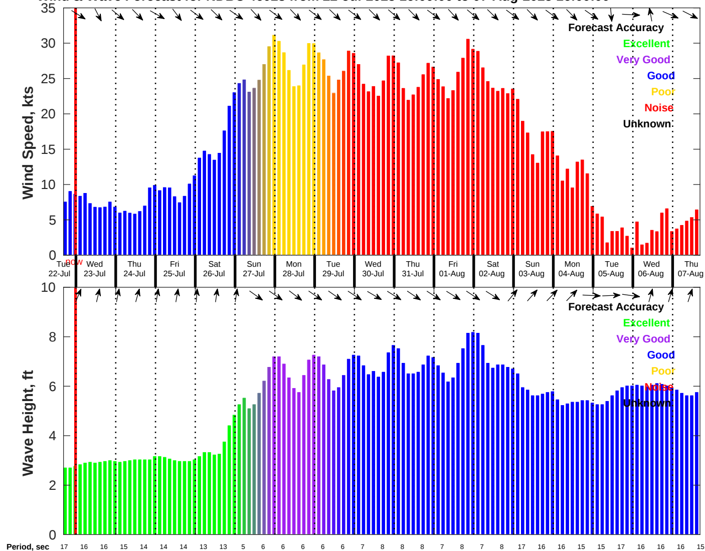
Wind & Wave Forecast for NDBC 46028 from 22-Jul-2025 16:00:00 to 07-Aug-2025 16:00:00
