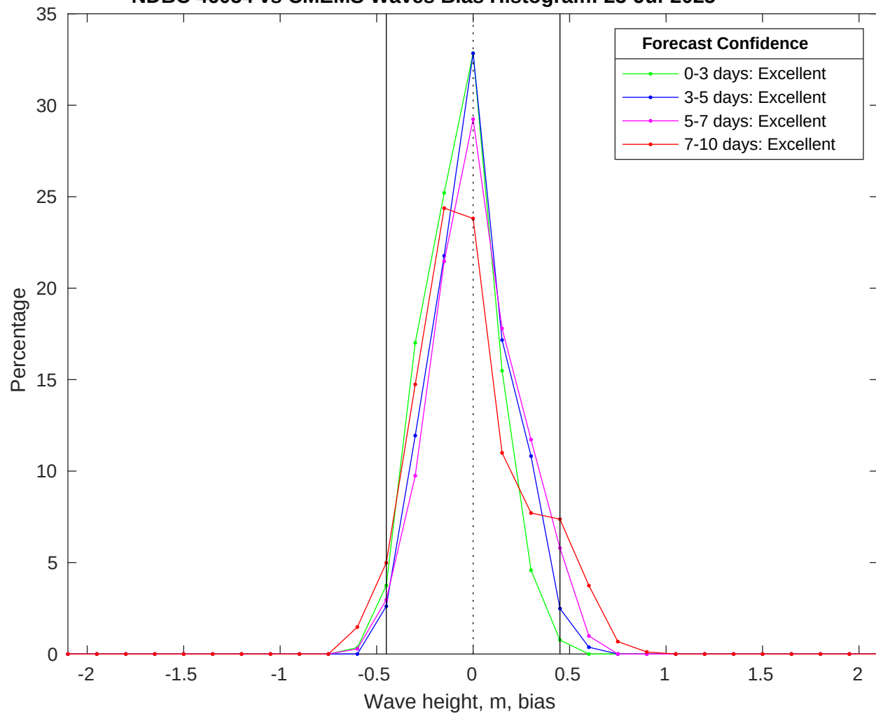
NDBC 46054 vs CMEMS Waves Bias Histogram: 23-Jul-2025
