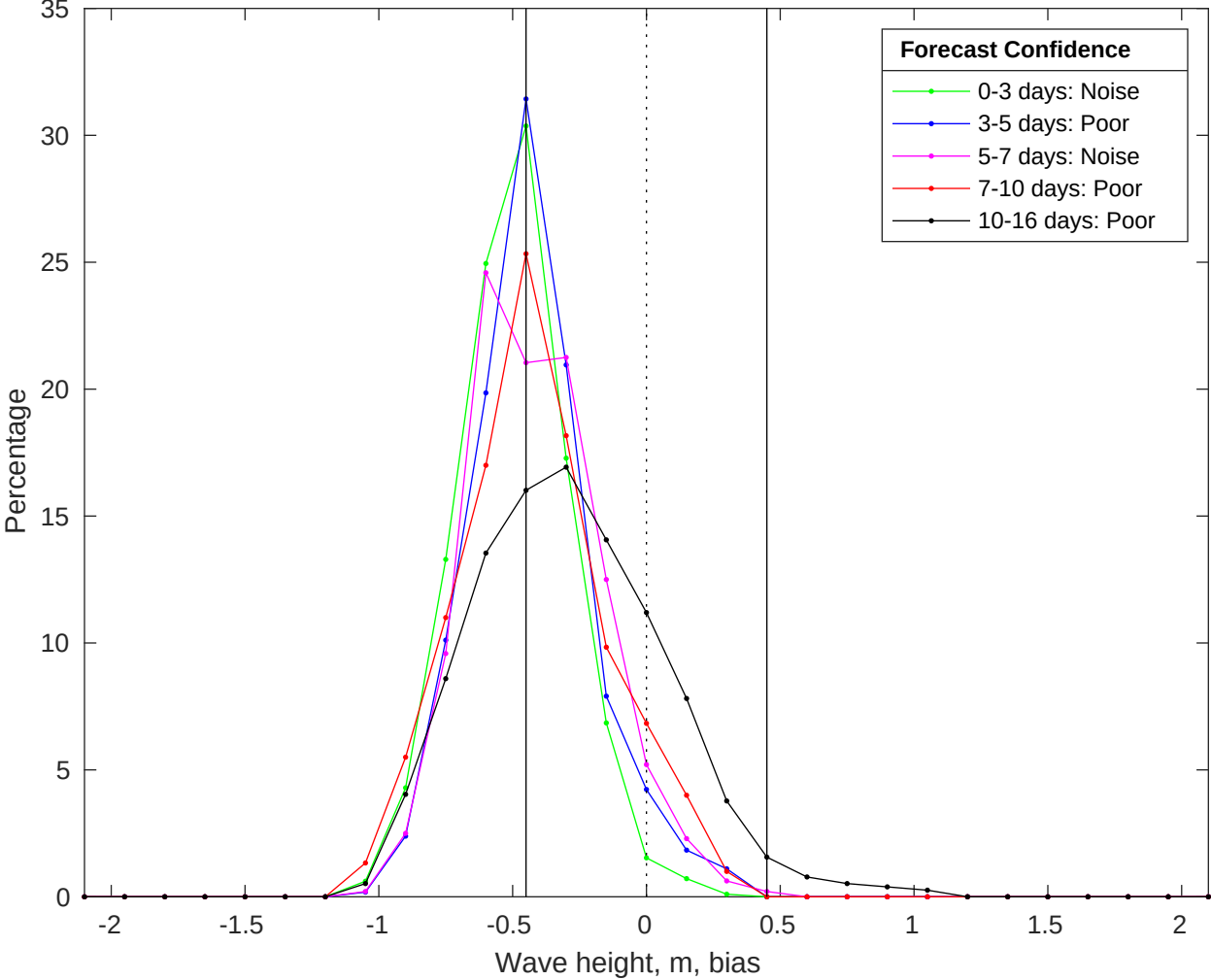
NDBC 46054 vs GFS Waves Bias Histogram: 23-Jul-2025
