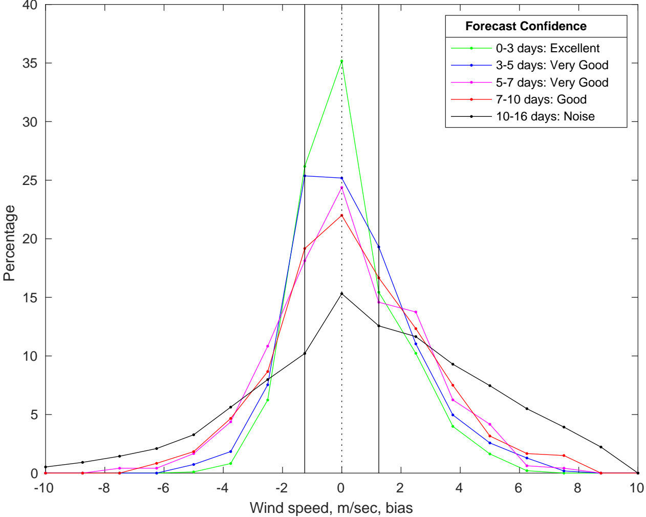
NDBC 46054 vs GFS Winds Bias Histogram: 23-Jul-2025
