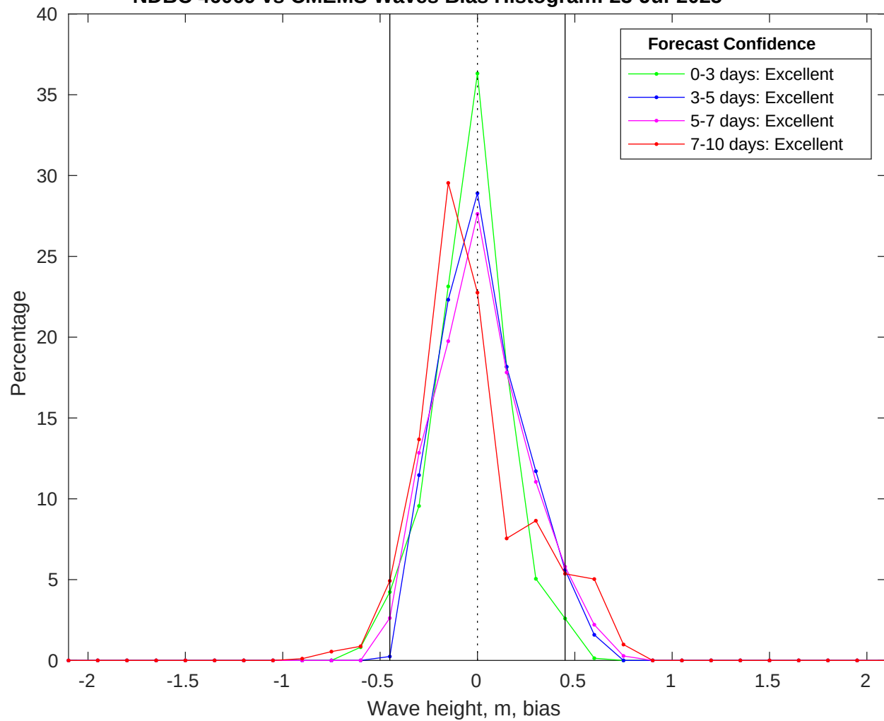
NDBC 46069 vs CMEMS Waves Bias Histogram: 23-Jul-2025
