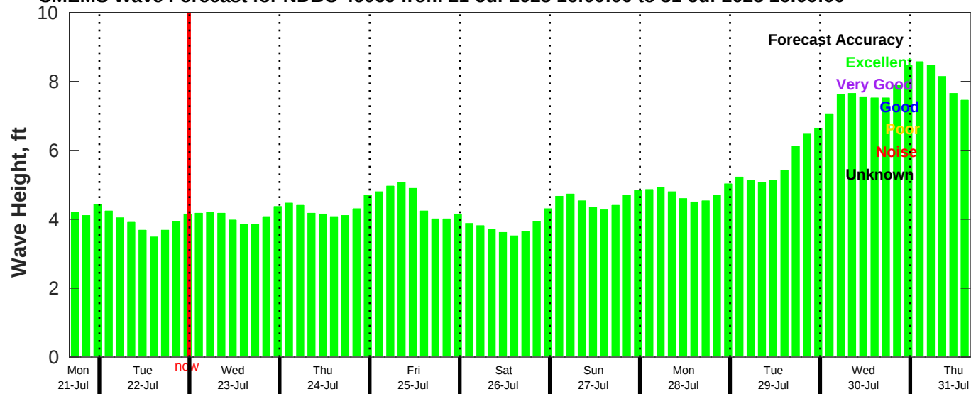
CMEMS Wave Forecast for NDBC 46069 from 21-Jul-2025 16:00:00 to 31-Jul-2025 16:00:00
