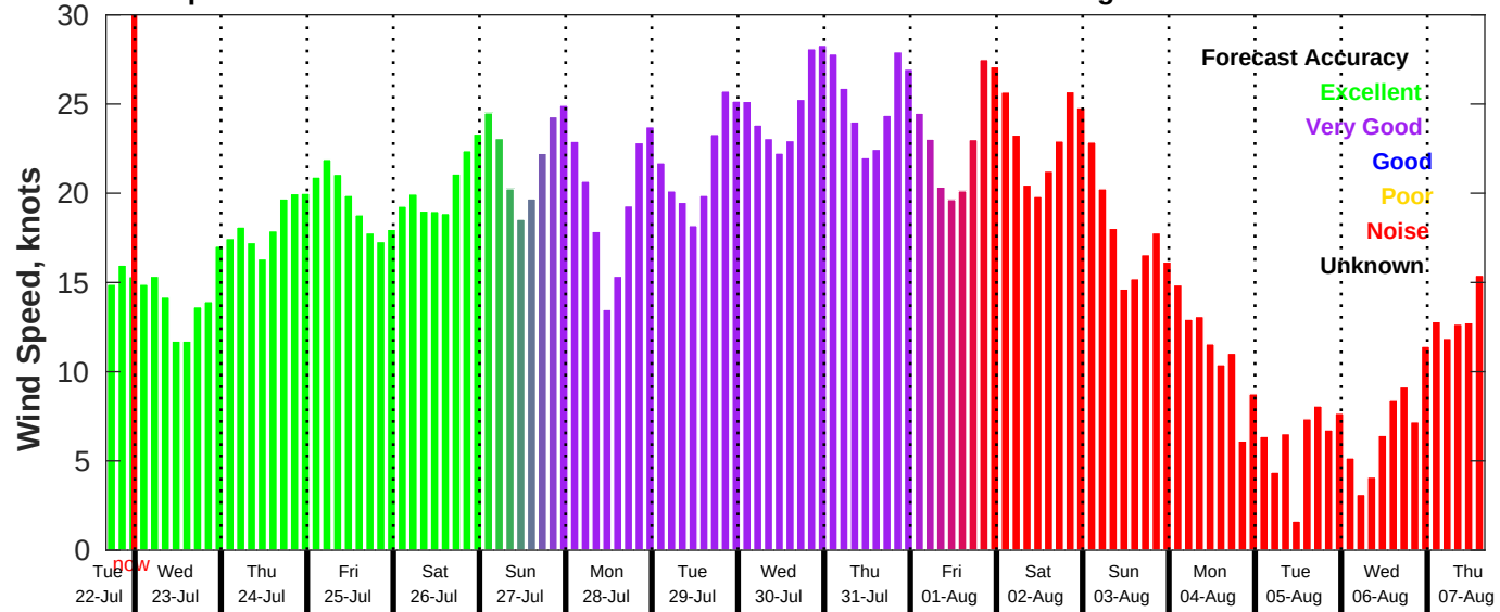
GFS Wind Speed Forecast for NDBC 46069 from 22-Jul-2025 16:00:00 to 07-Aug-2025 16:00:00
