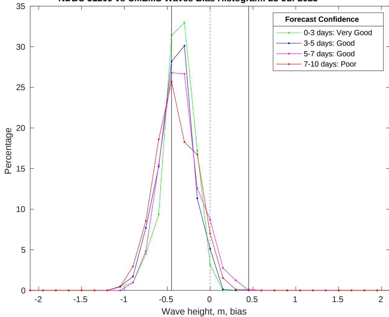
NDBC 51209 vs CMEMS Waves Bias Histogram: 23-Jul-2025
